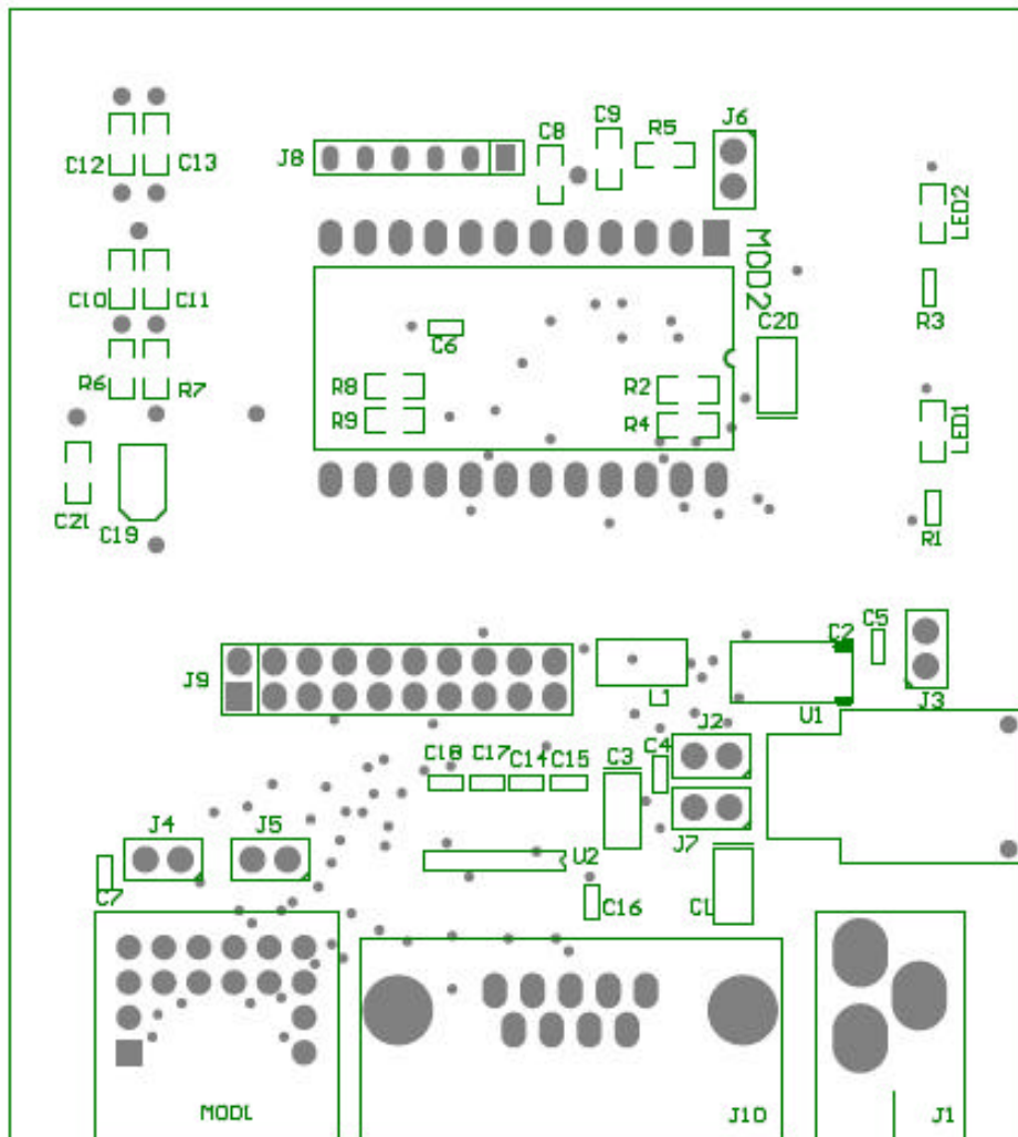
Ver 1.8 PCB component overlay
